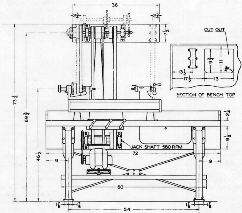
Overhead Countershaft Drive with Auxiliary Countershaft Attachment and Hand Belt Shifters.
