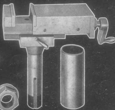
Vise for Eccentric Slide Rest
