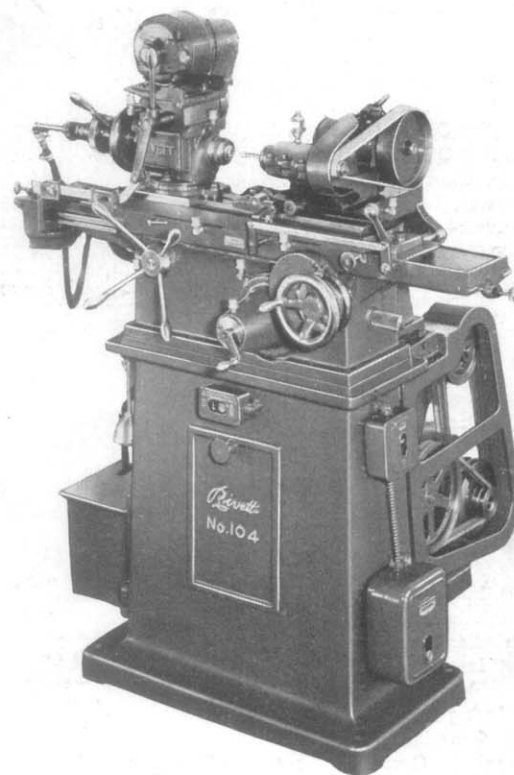
Rivett No. 104 Internal-External Grinder, 2" or 4" Power Reciprocation, 8" Swing.
