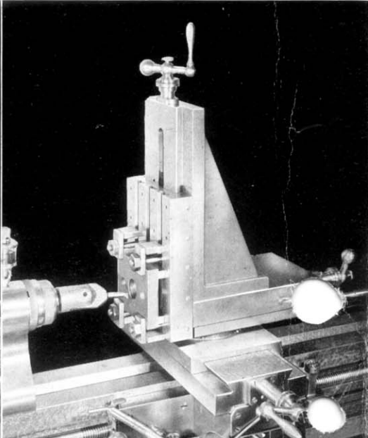
Fig. 3—Jig boring on "608"
