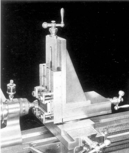
Fig. 2—Milling dovetail on "608"
