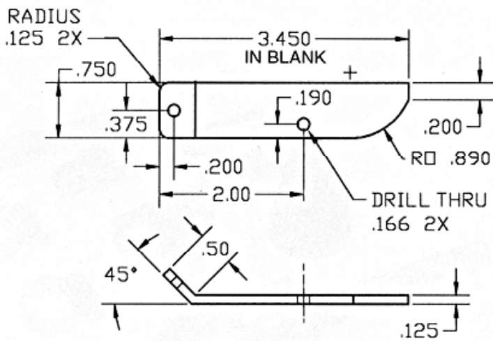
⑥ TRIP LEVER mat'l - 6061 aluminum plate
