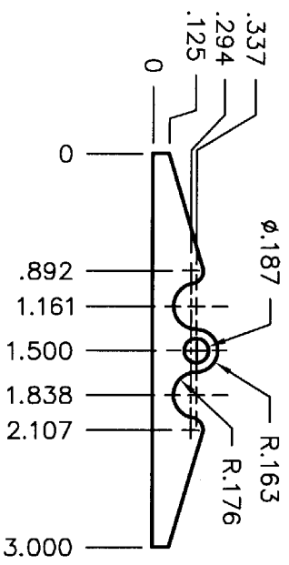
8 VALVE LEVER ALUMINUM 1 REQ'D.
