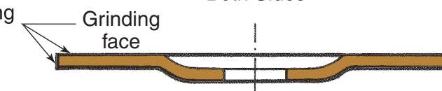
Type 27 Depressed Center
