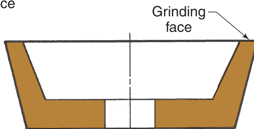
Type 11 Flaring Cup Wheel
