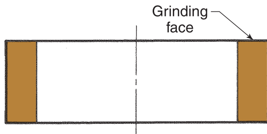
Type 2 Cylinder Wheel
