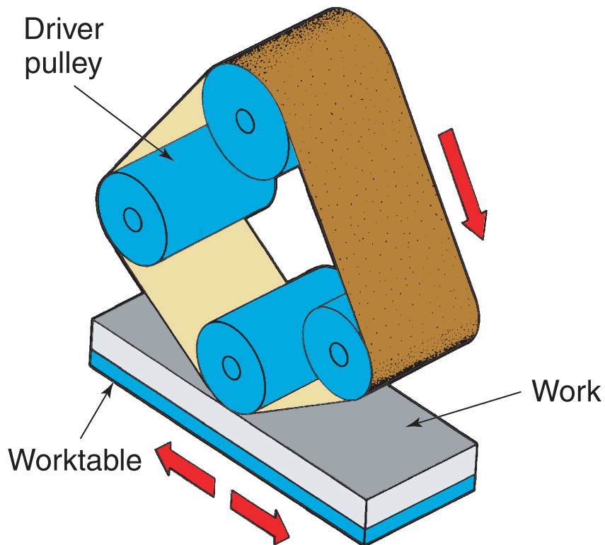
Abrasive Belt Machining
