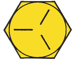
Customary (inch) Bolts
