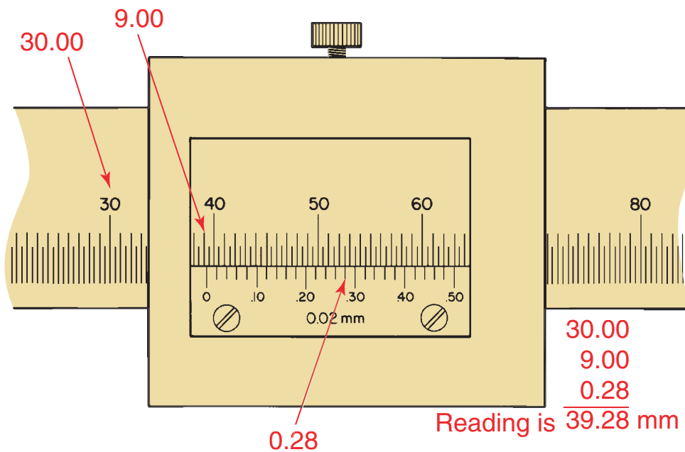
25-Division Metric Vernier Scale
