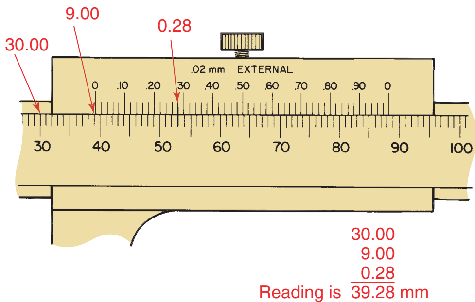
50-Division Metric Vernier Scale
