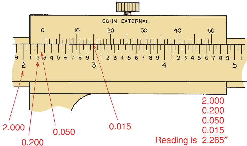
50-Division Vernier
